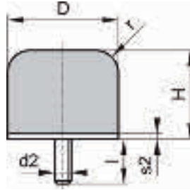
KRAN-GUMMI-METALL-PUFFER
